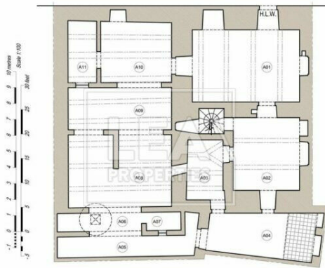
01 Existing Basement Level Plan
