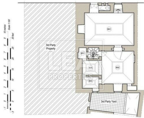
02 Existing Ground Floor Level Plan
